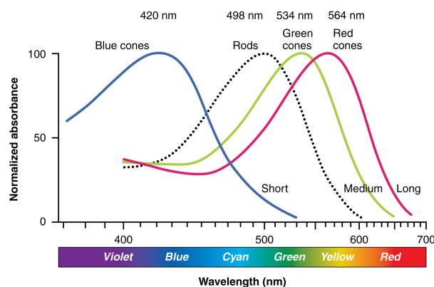
Normalised absorption spectra of the three human photopsins and of human rhodopsin (dashed).
